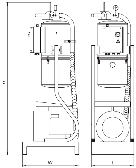
Vacuum unit with CF filters
