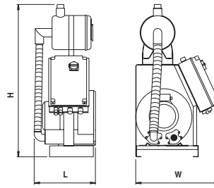
Vacuum unit with FZ filter
