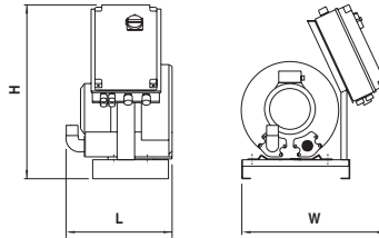
Vacuum unit
